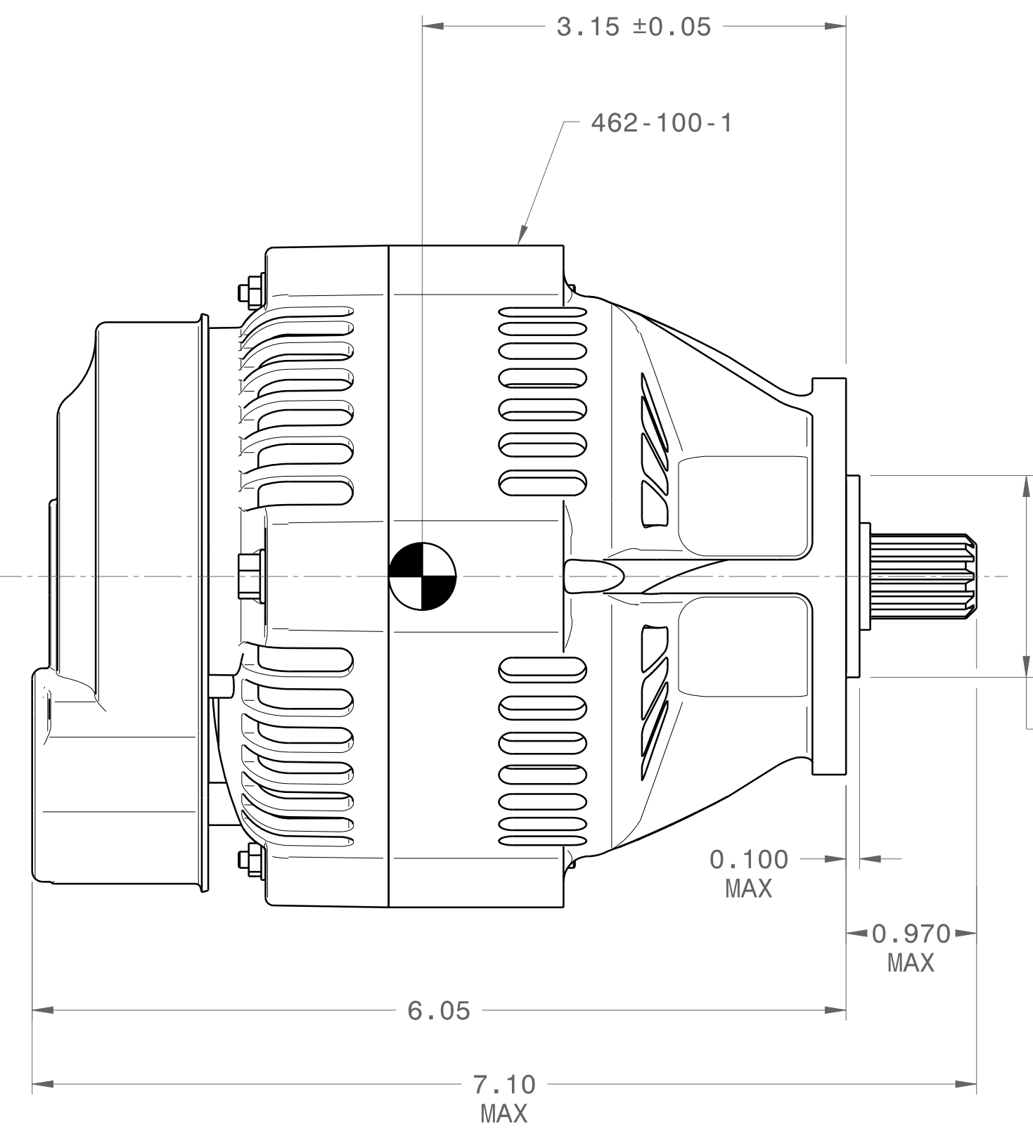
-1 ALTERNATOR SIDE VIEW SCALE 1:1
